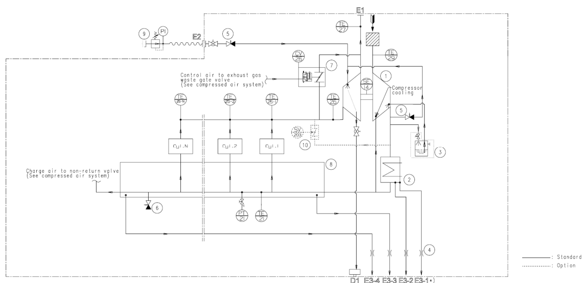
Figure 9.3 Diagram for combustion and exhaust gas system (B92-355597-2.0)
