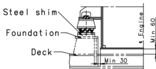
Figure 2.5 Resilient mounting
