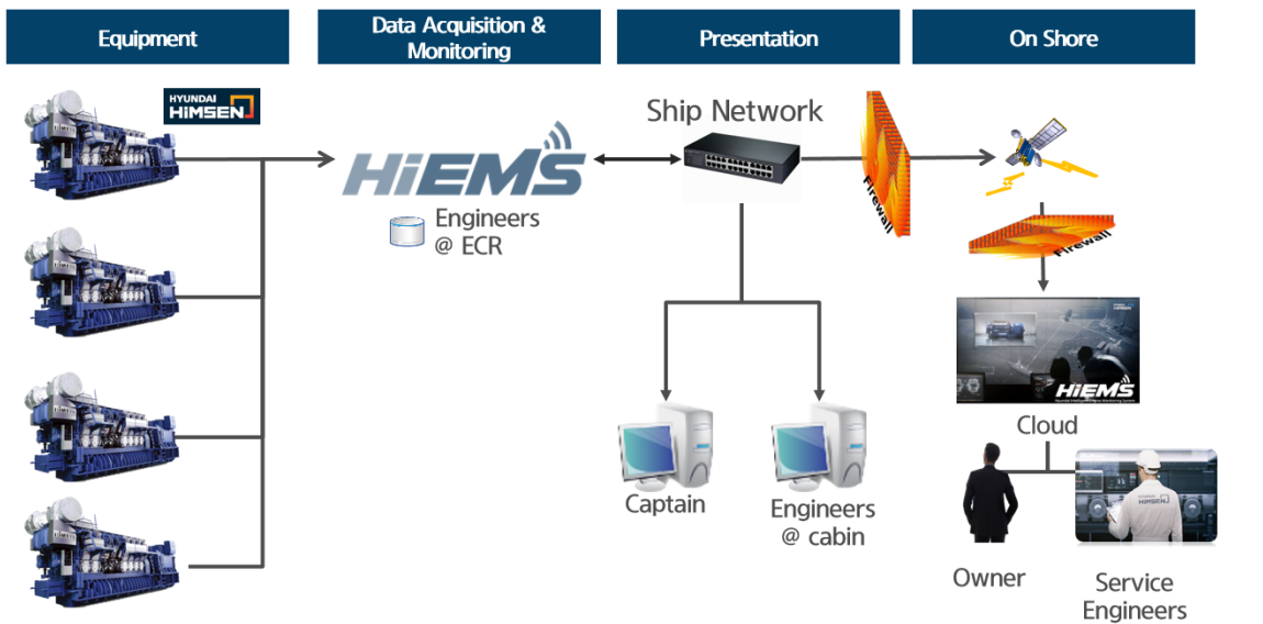
Figure 5.24 HiMEMS configuration and network
