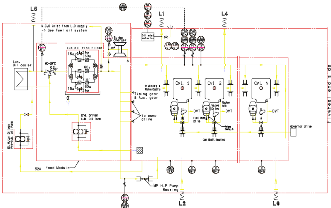
Figure 7.1 Diagram for internal lubricating oil system
