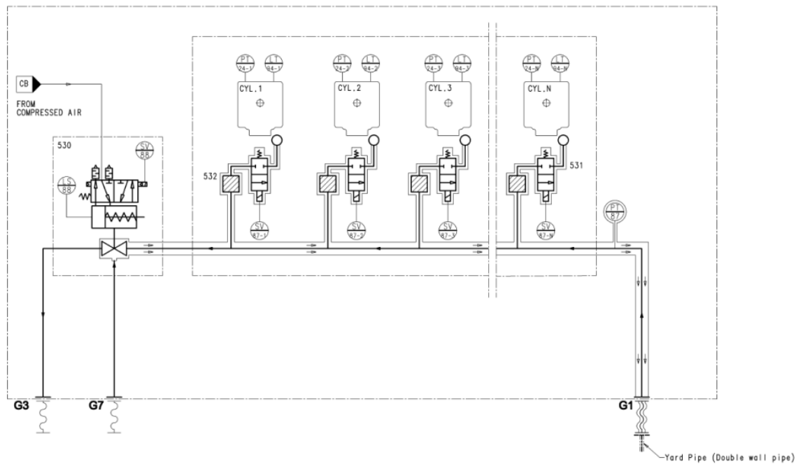
Figure 6.5 Diagram for internal fuel gas system
