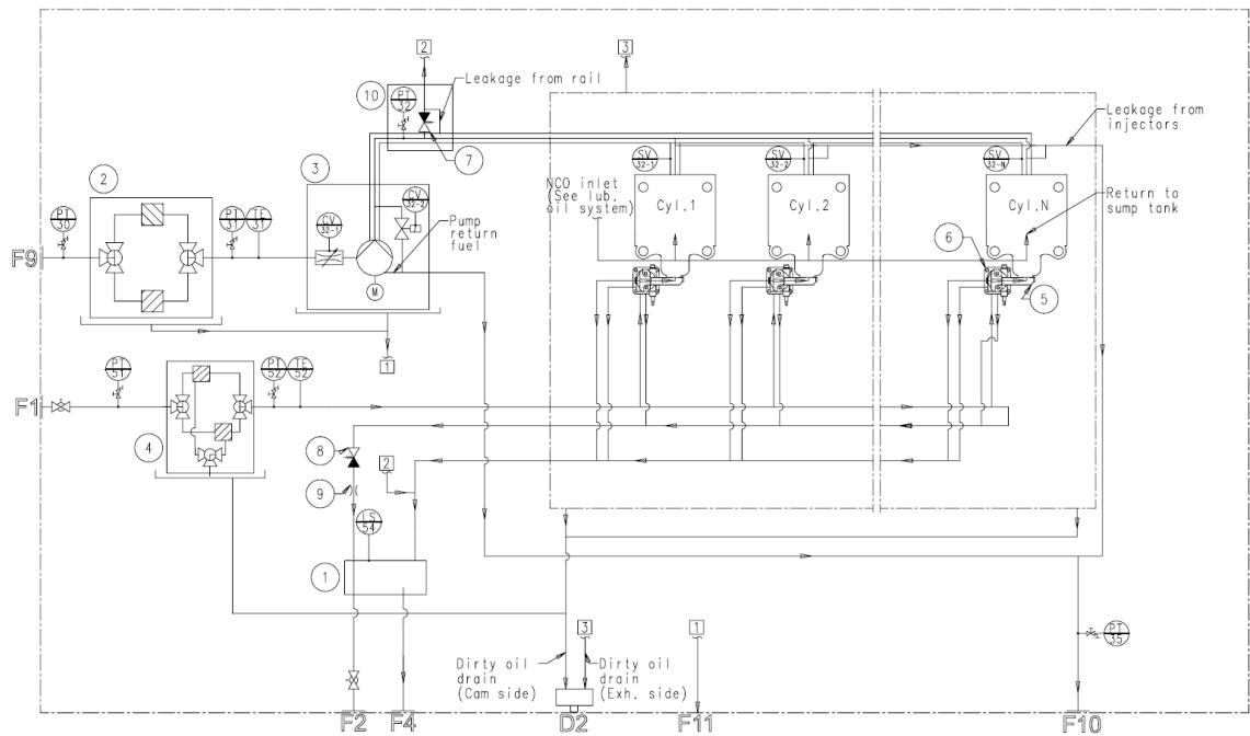
Figure 6.1 Diagram for Internal fuel oil system (B92-310324-0.0)
