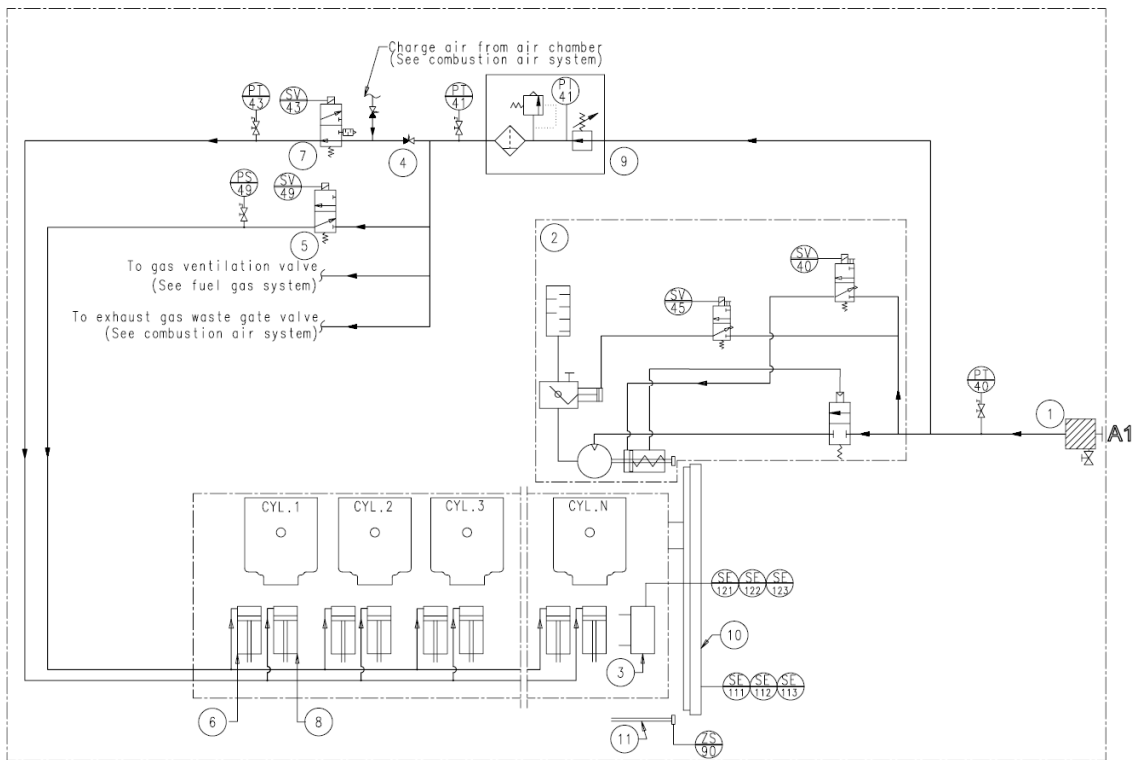
Figure 9.1 Diagram for internal compressed air system (B92-310327-6.0)
