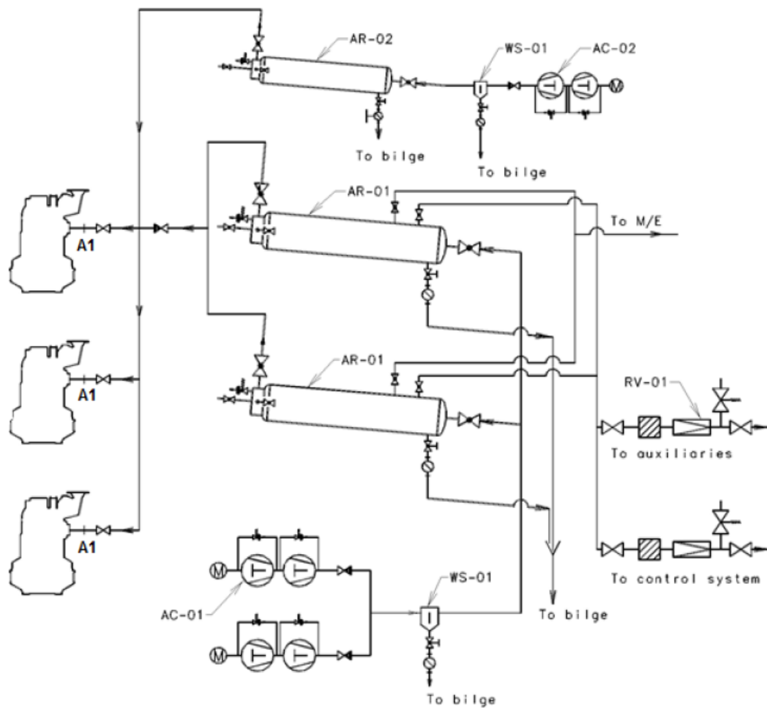
Figure 9.2 Diagram for external compressed air system
