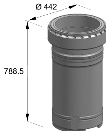
Cylinder liner (Weight : approx. 189.96 kg)
