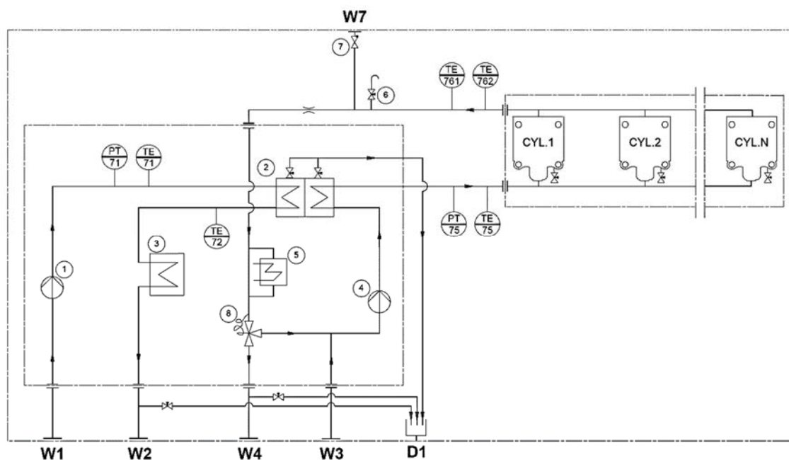
Figure 8.1 Diagram for internal cooling water system [BP0061793-0.4]
