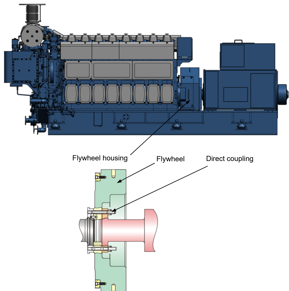
Figure 9.9 Direct coupling outline
