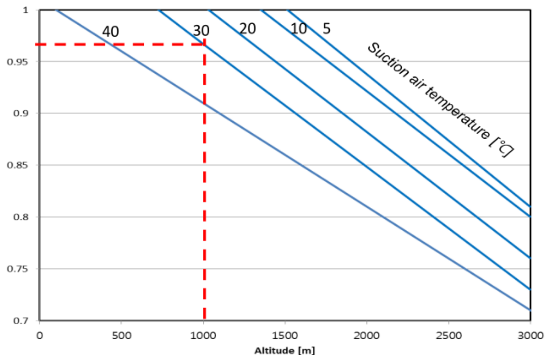
Figure 3.6 De-rating due to suction air temperature and altitude
