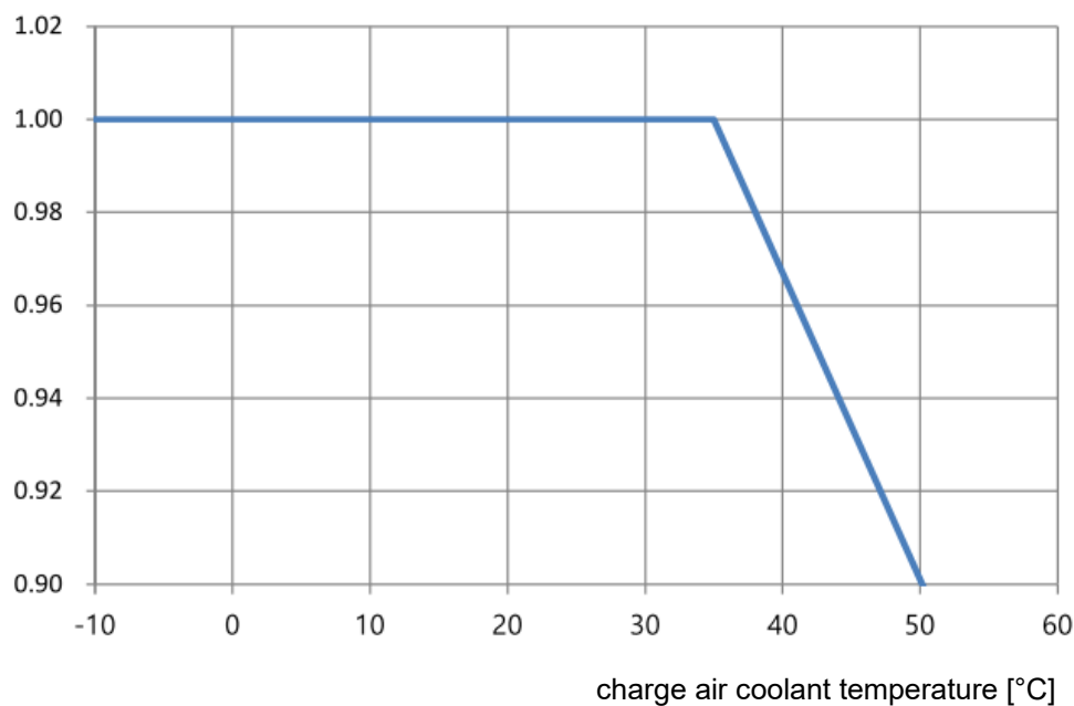
Figure 3.9 De-rating due to charge air coolant temperature
