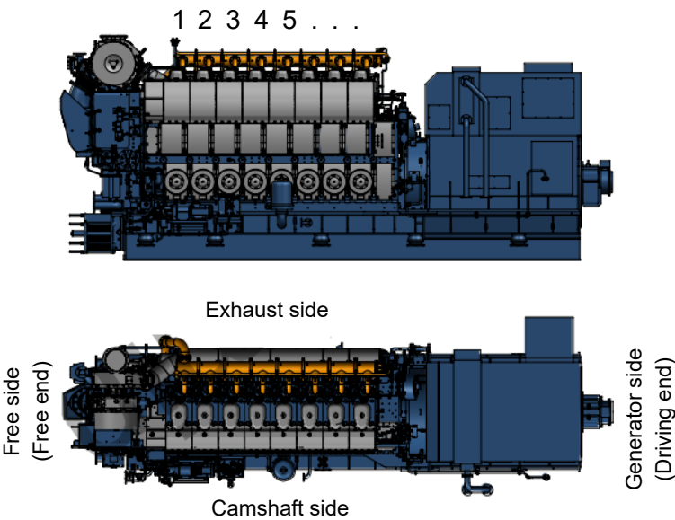
Figure 1.1 Cylinder numbering
