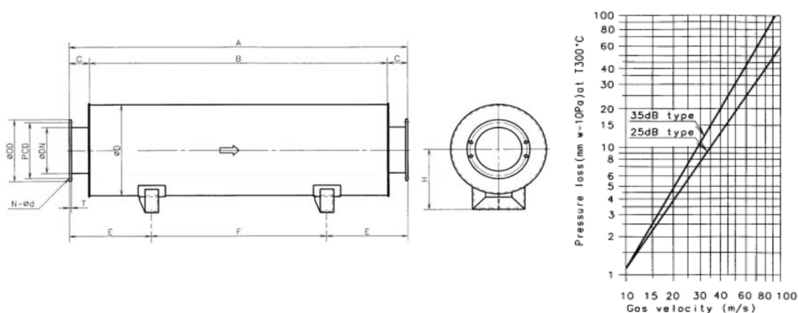
Figure 9.8 Exhaust gas silencer (25 dB type).
