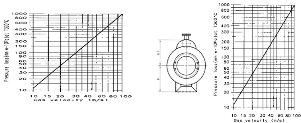
Figure 9.7 Exhaust gas silencer (35 dB type).
