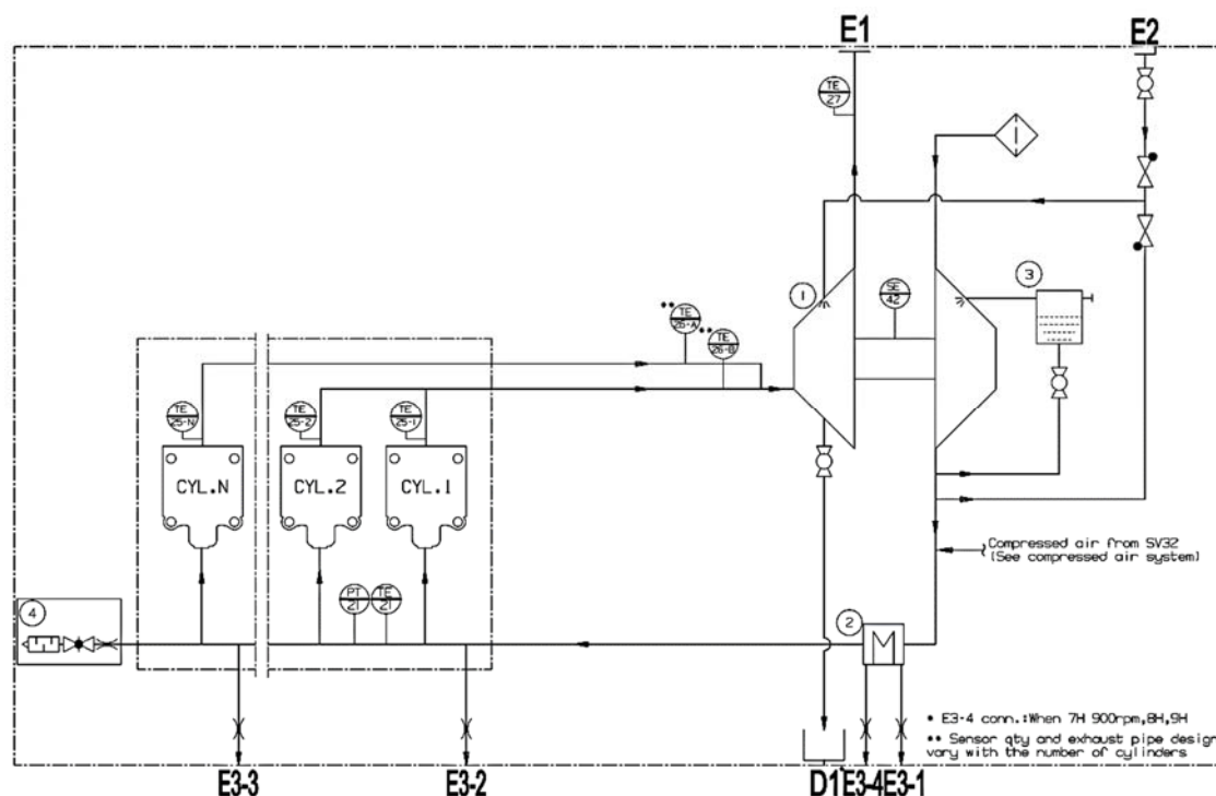
Figure 9.3 Diagram for combustion and exhaust gas system [B92-128965-0.0]
