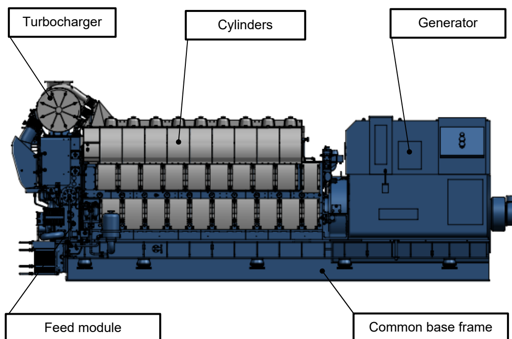
Figure 2.2 Engine design outline
