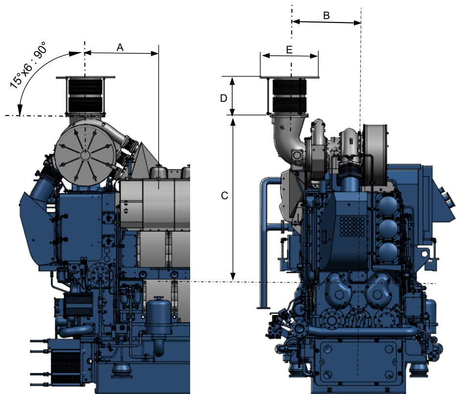
Figure 9.4 External exhaust gas pipe connection.
