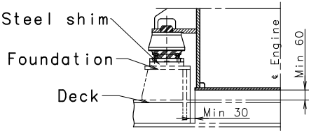
Figure 2.5 Resilient mounting
