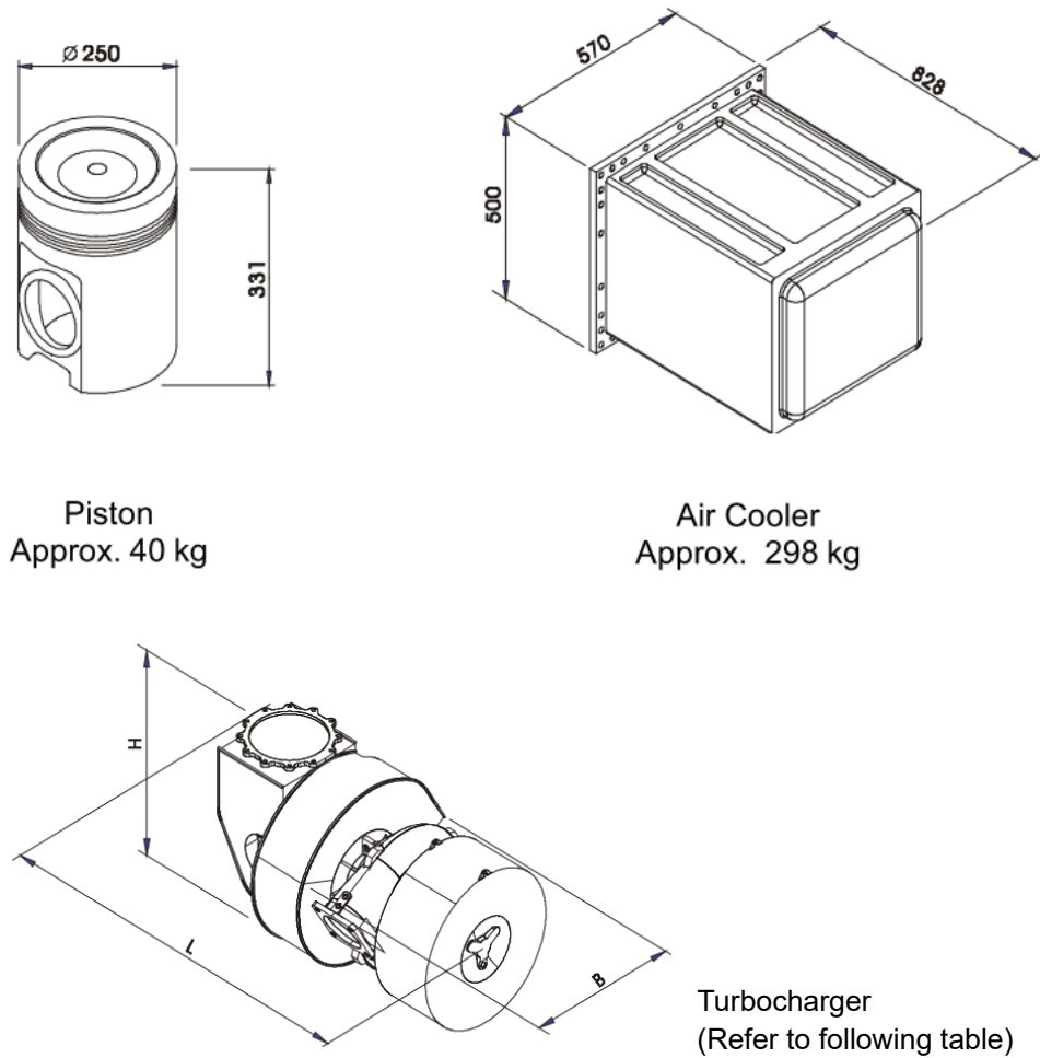
Figure 10.1 Heavy parts dimension and weight.
