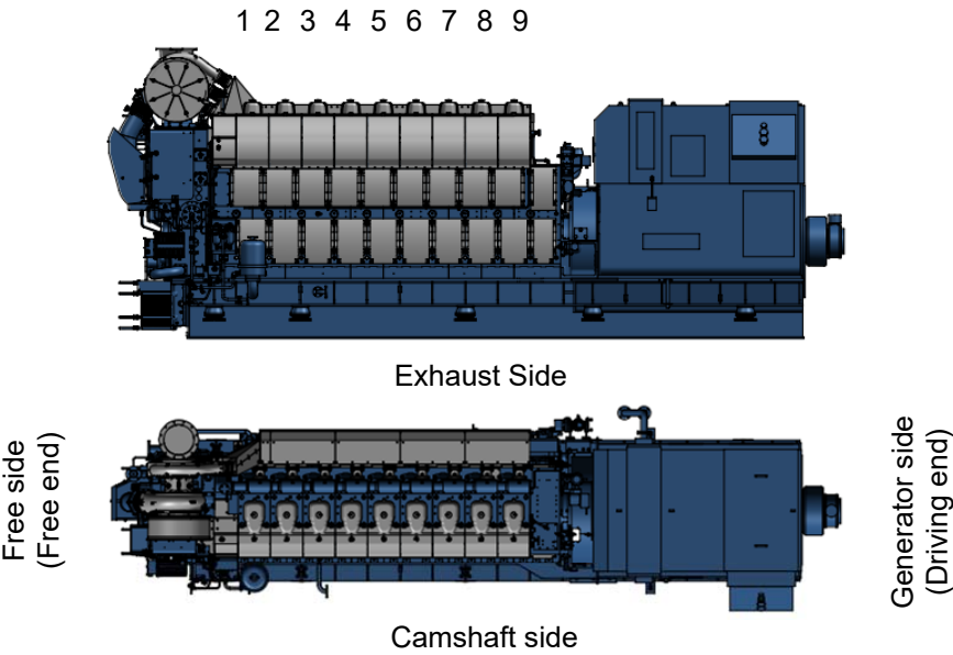
Figure 1.1 Cylinder numbering
