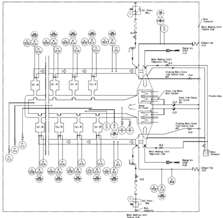
Figure 9.3 Diagram for combustion and exhaust gas system [B92-328929-9.0]
