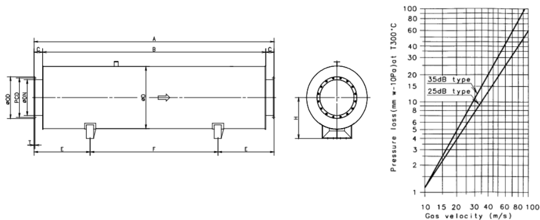
Figure 9.9 Exhaust gas silencer (25 dB type).
