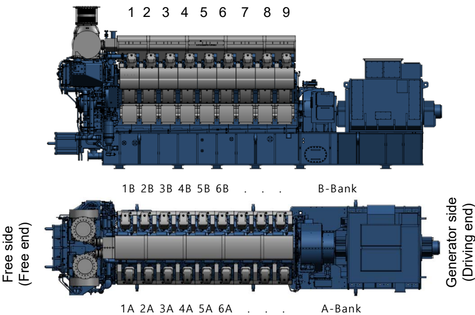
Figure 1.1 Cylinder numbering
