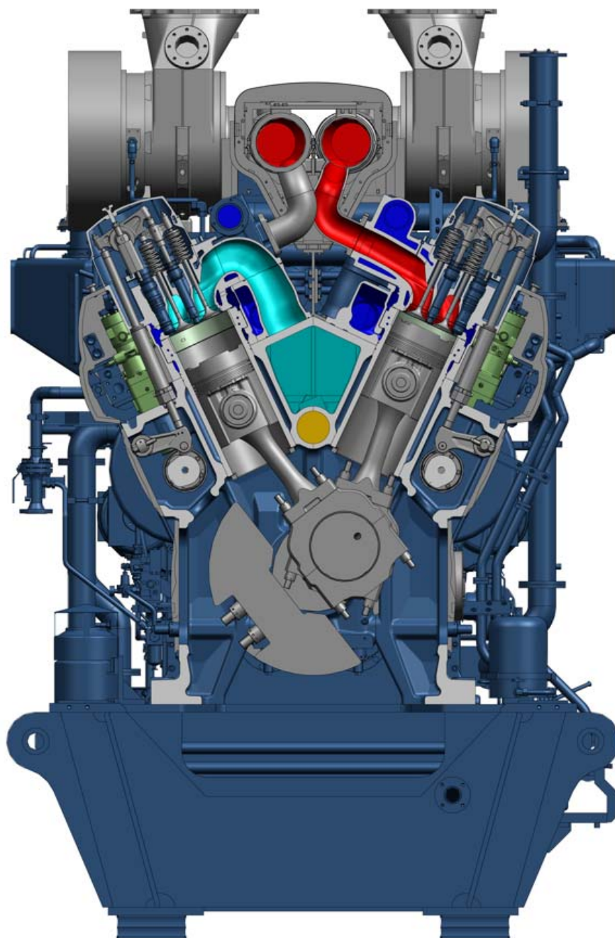
Figure 2.1 Engine cross section
