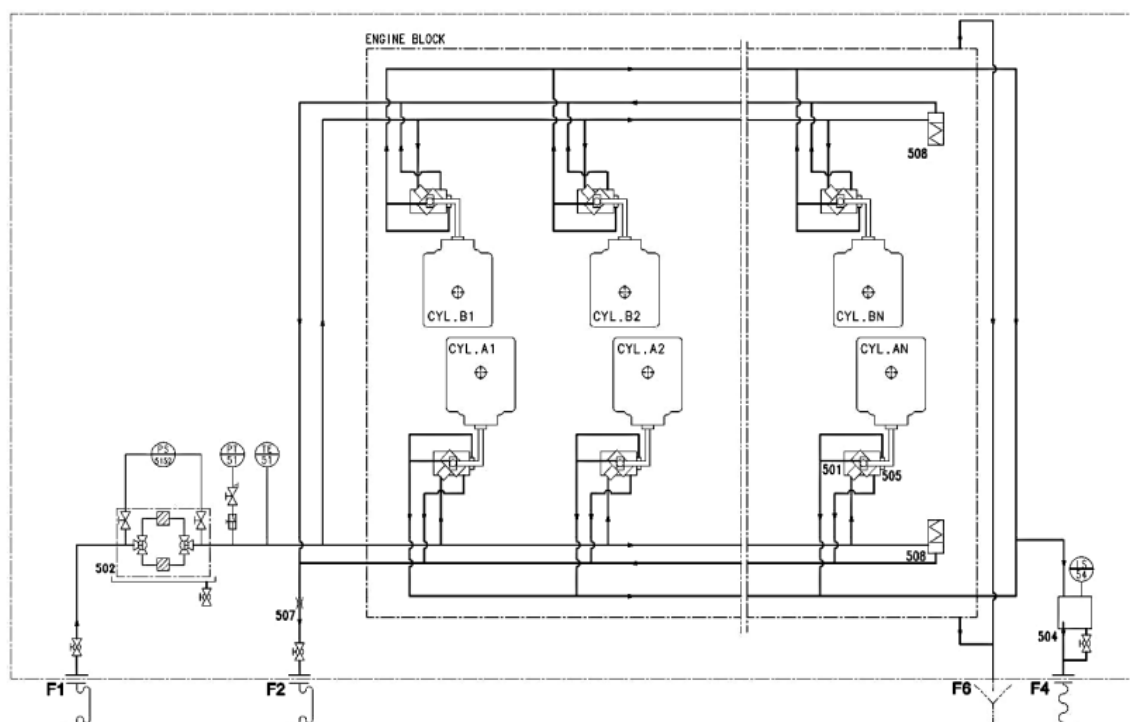
Figure 6.1 Diagram for Internal fuel oil system
