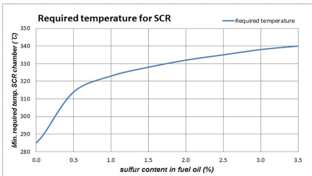
Figure 9.6 Minimum required exhaust gas temperature for SCR operation
