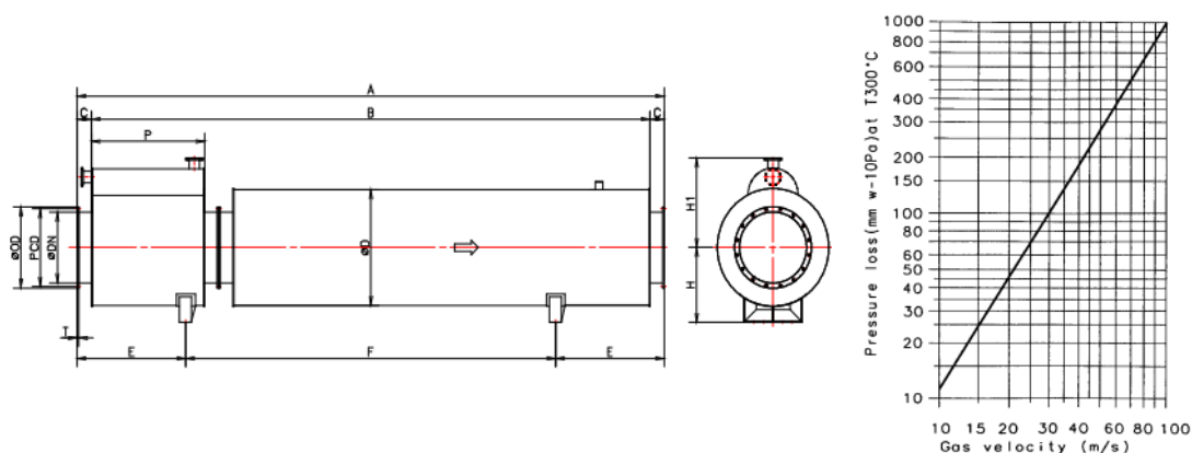
Figure 9.8 Exhaust gas silencer (35 dB type).
