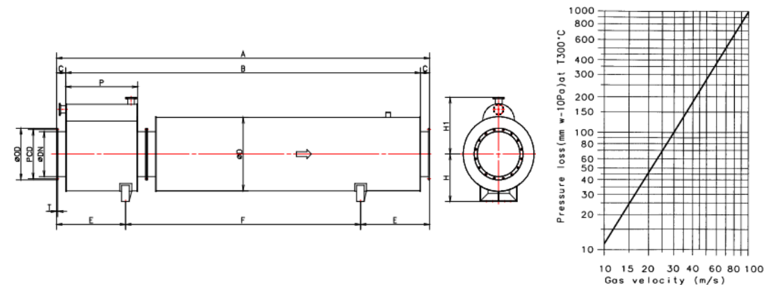
Figure 9.7 Exhaust gas silencer (25 dB type)
