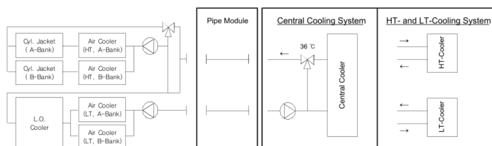
Figure 3.1 Cooling system arrangement
