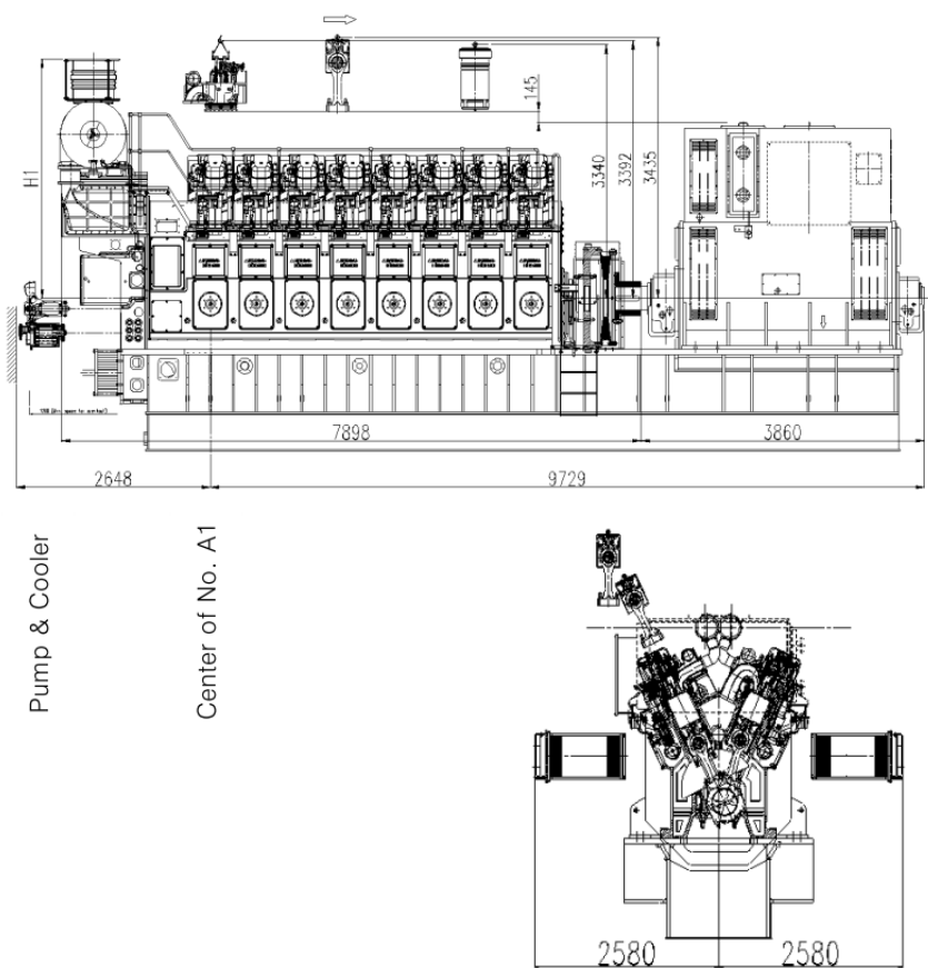
Figure 2.7 Overhaul dimension
