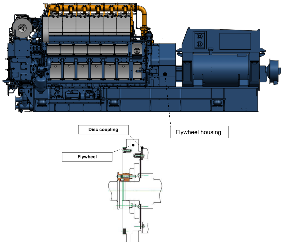
Figure 9.8 Disc coupling outline
