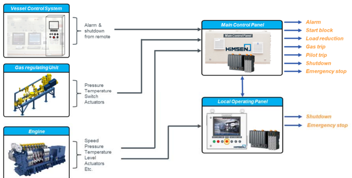
Figure 5.10 H22CDF engine safety function layout
