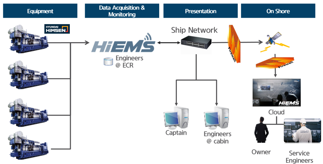
Figure 5.24 HiEMS configuration and network
