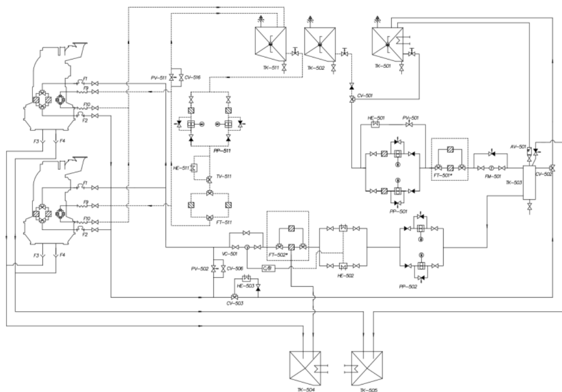
Figure 6.2 Diagram for heavy fuel oil system
