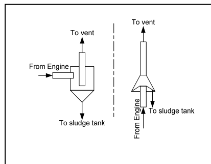
Figure 7.6 an example of condensation trap
