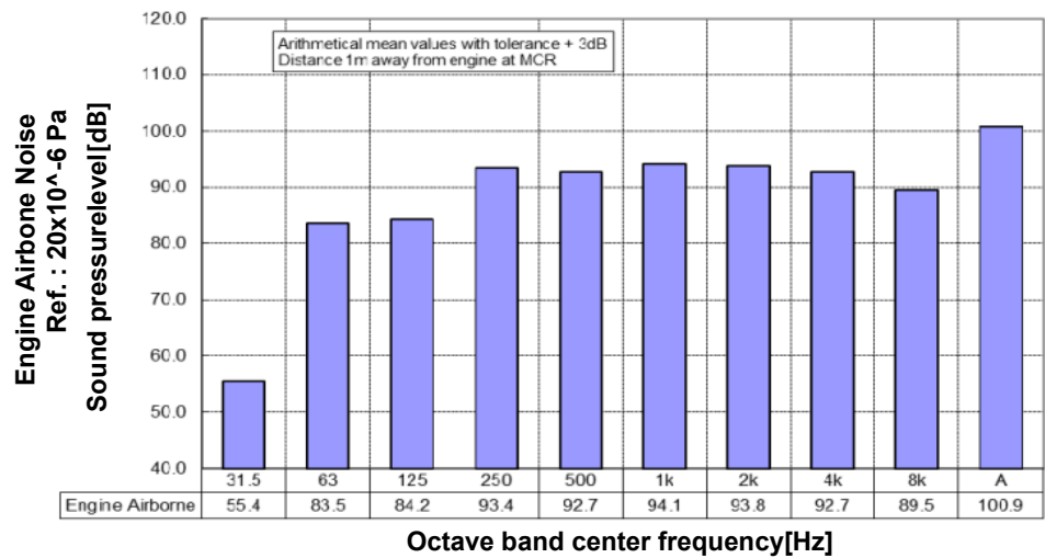
Figure 4.1 Engine air airborne noise level (Diesel mode)
