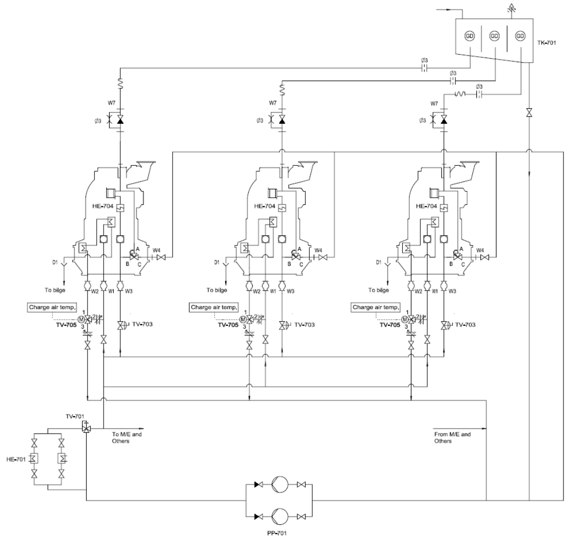
Figure 8.3 Diagram for external cooling water system with electric pre-heating element (B92-325134-8.1)
