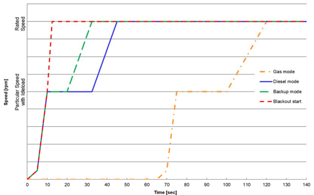
Figure 5.3 Engine start at different fuel mode
