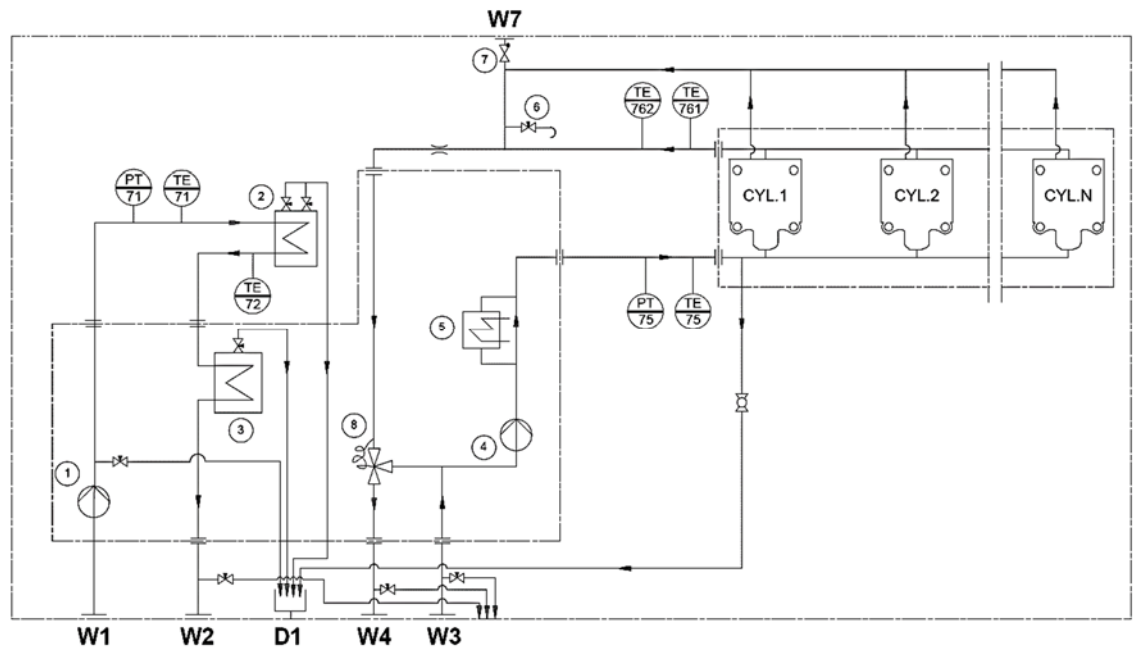
Figure 8.1 Diagram for internal cooling water system [BP0068578-0.0]
