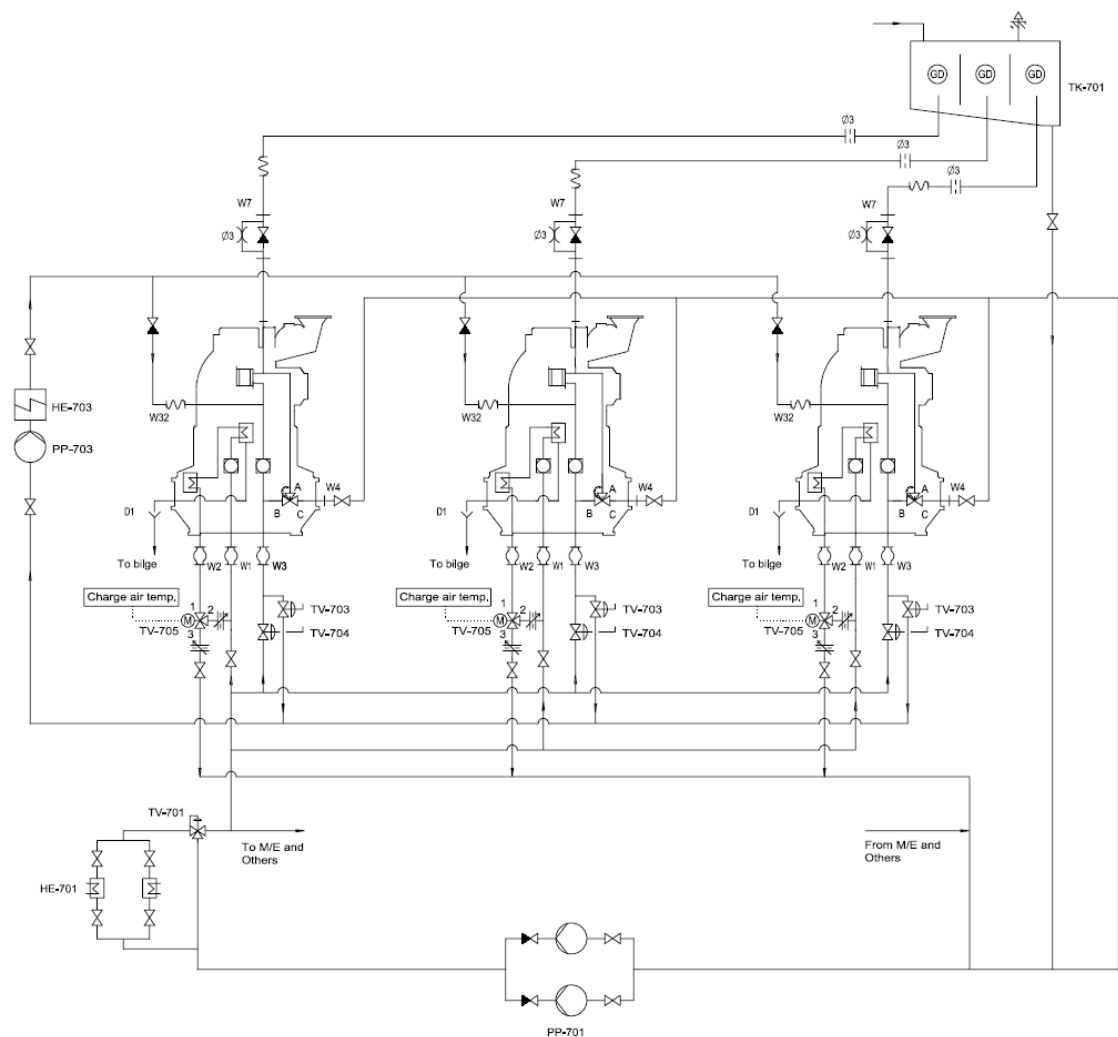
Figure 8.4 Diagram for external cooling water system with pre-heating unit (B92-325135-0.3)
