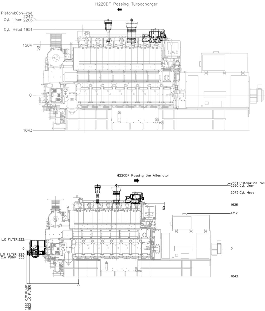
Figure 2.7 Overhaul dimension
