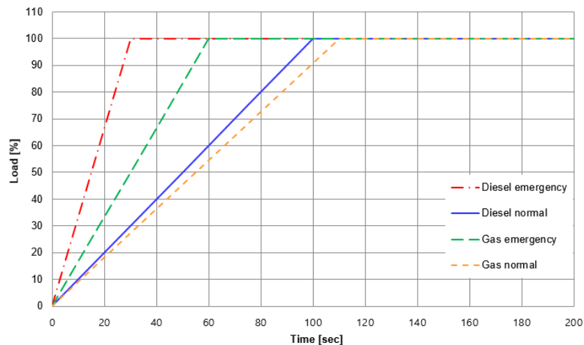
Figure 5.5 Engine load up capacity in ramp
