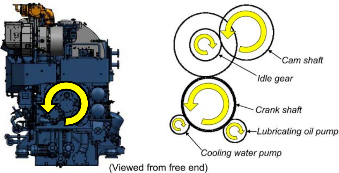
Figure 1.2 Direction of engine rotation
