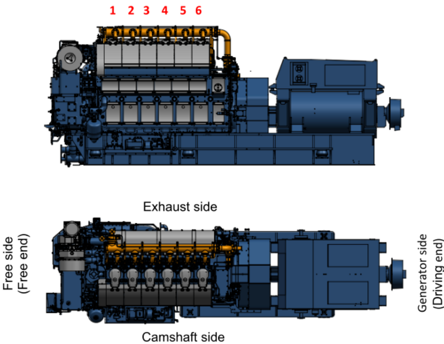
Figure 1.1 Cylinder numbering
