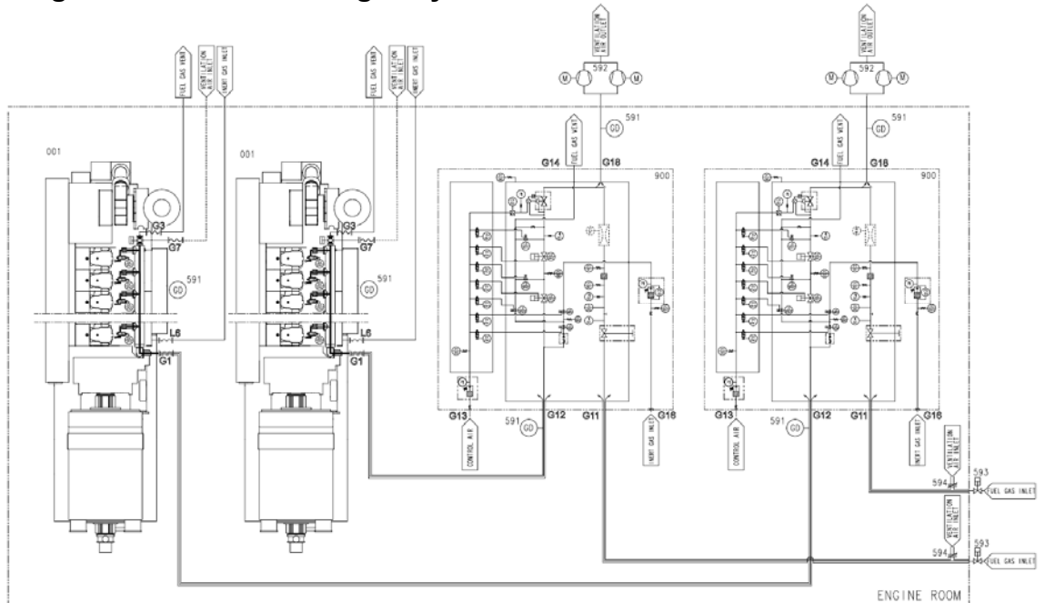
Figure 6.6 Diagram for external fuel gas system (BH1-104579-4.3)
