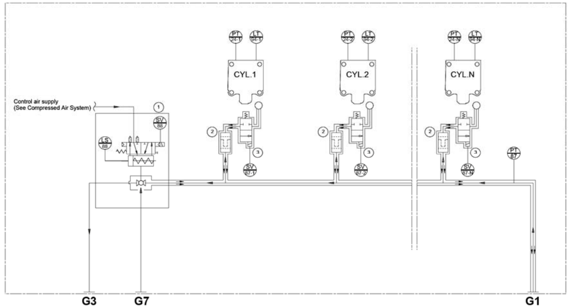
Figure 6.5 Diagram for internal fuel gas system [BP0061847-0.4]
