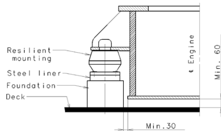
Figure 2.5 Resilient mounting
