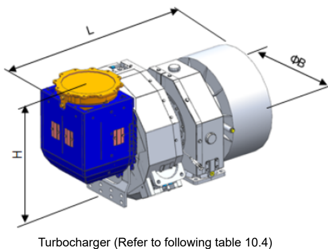
Figure 10.1 Heavy parts dimension and weight.
