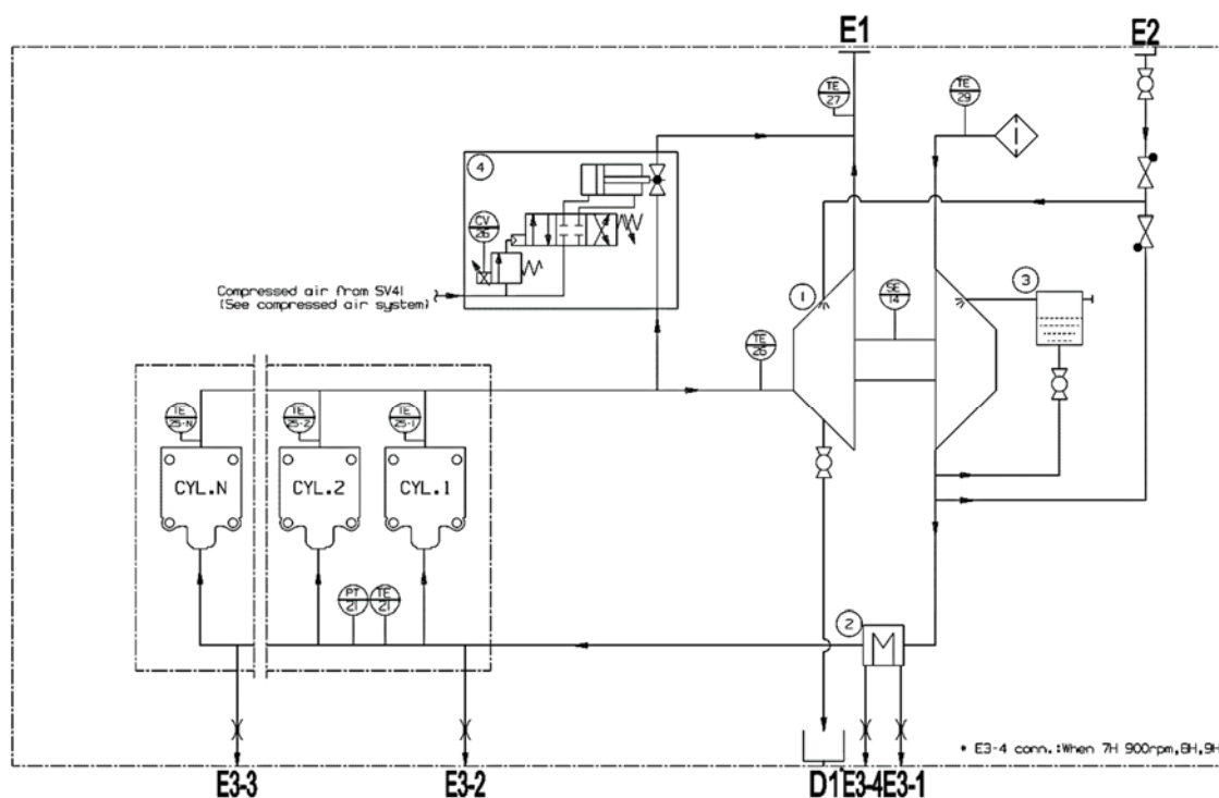
Figure 9.3 Diagram for combustion and exhaust gas system [B92-128961-2.1]
