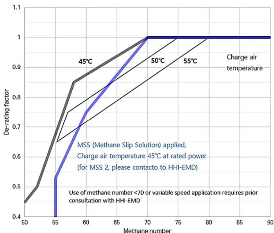
Figure 3.7 Minimum de-rating due to charge air temperature and methane number
