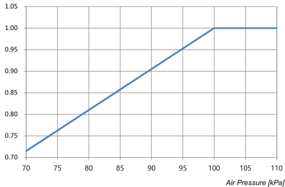
Figure 3.11 De-rating due to air pressure
