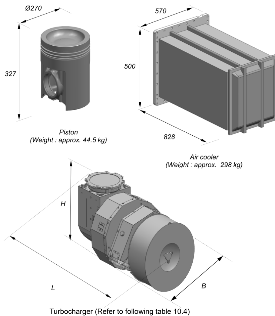
Figure 10.1 Heavy parts dimension and weight.
