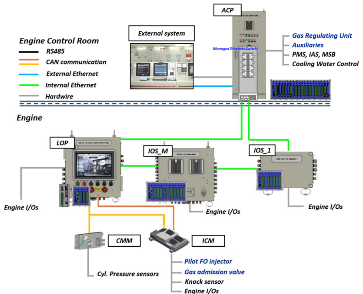
Figure 5.14 HiMSEN DF Engine Control System overview
