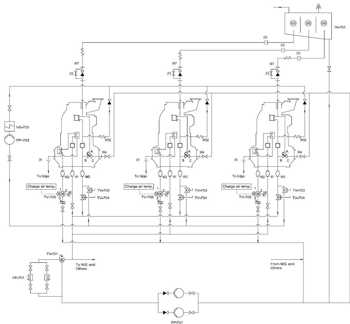
Figure 8.3 Diagram for external cooling water system with pre-heating unit (B92-329037-3.2)
