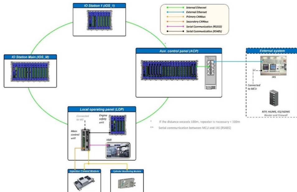
Figure 5.25 Communication diagram for HiMECS-AE
