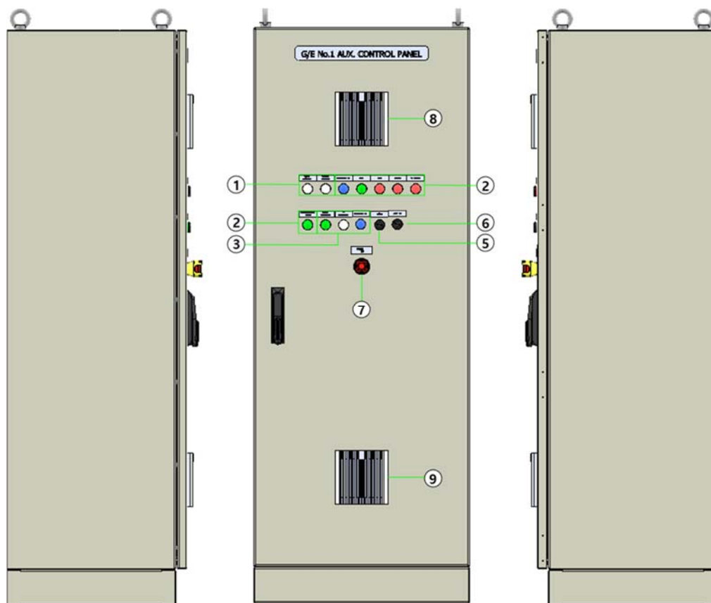
Figure 5.21 Auxiliary Control Panel
