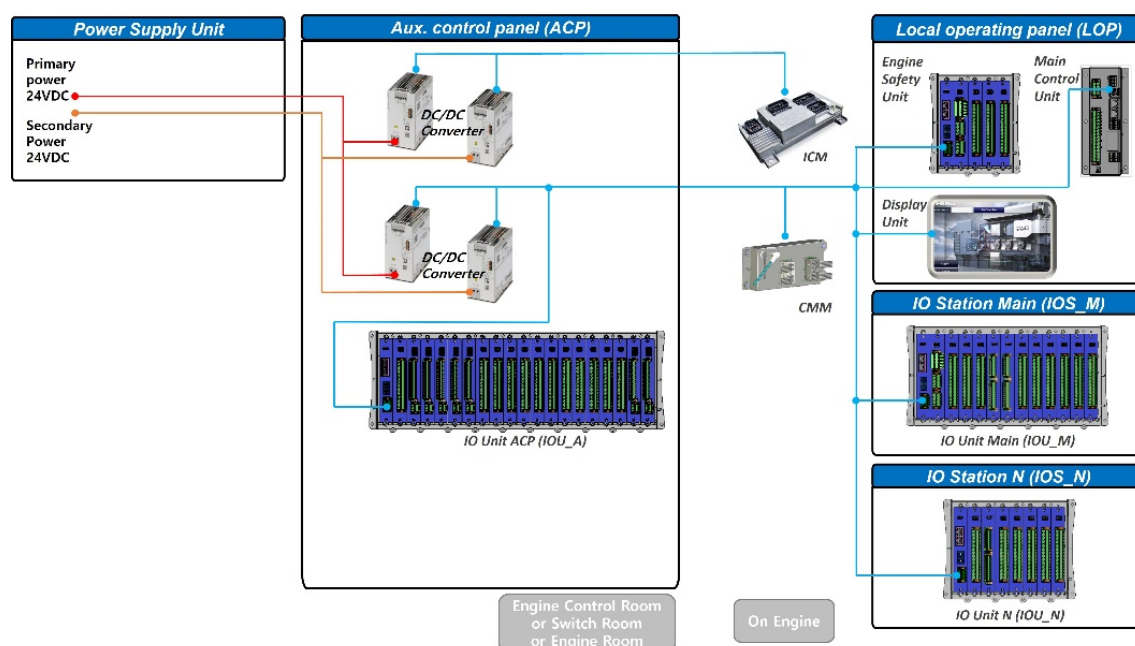
Figure 5.26 Power distribution diagram for HiMECS-AE
