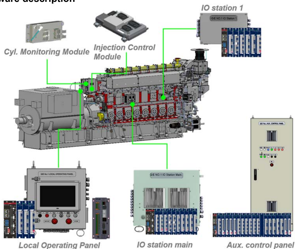
Figure 5.15 Arrangement of HiMECS-AE for H35DF
