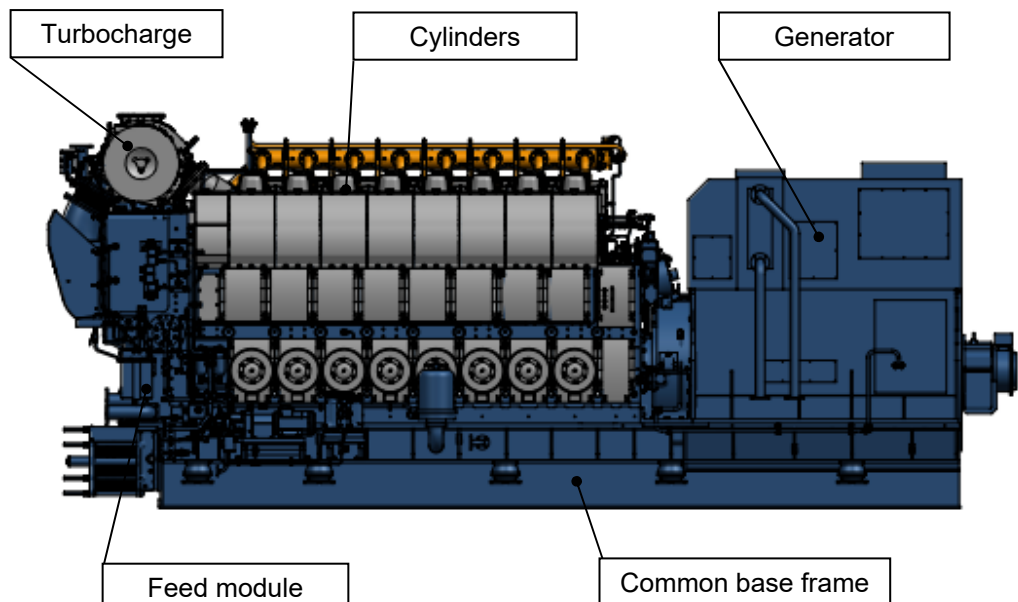
Figure 2.2 Engine design outline
