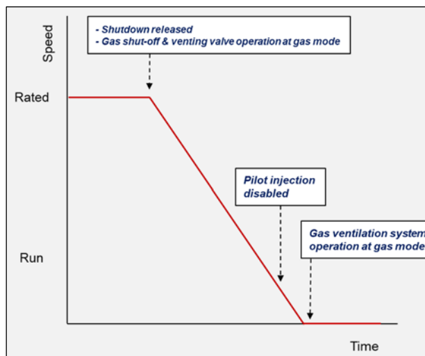
Figure 5.11 Shutdown sequence
