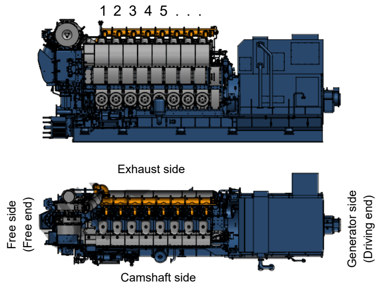
Figure 1.1 Cylinder numbering
