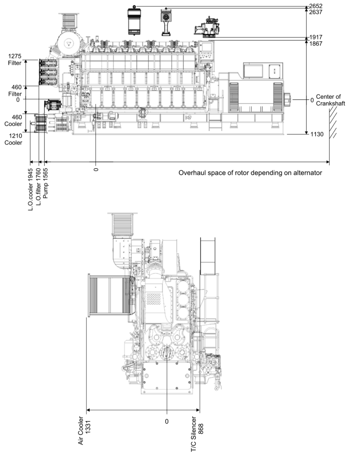
Figure 2.7 Overhaul dimension
