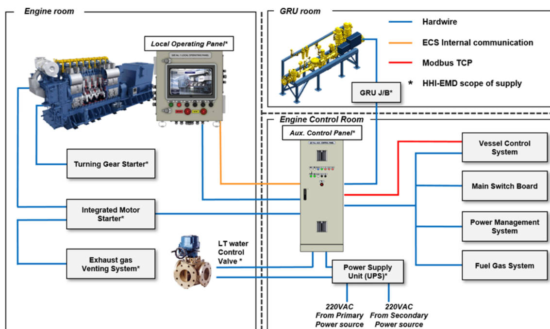
Figure 5.24 HiMSEN DF ECS external interface (system schematic)
