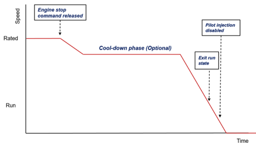
Figure 5.10 Engine normal stop sequence
