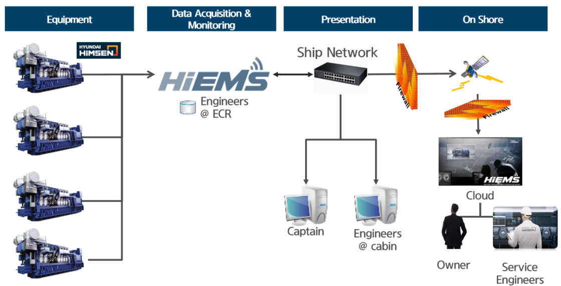
Figure 5.27 HiEMS configuration and network
