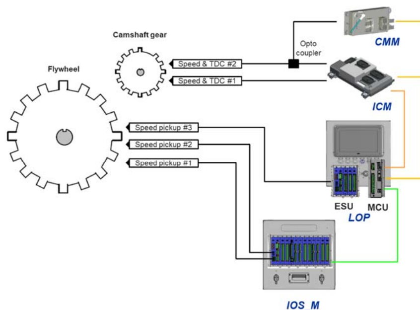
Figure 5.22 Speed measurement configuration
