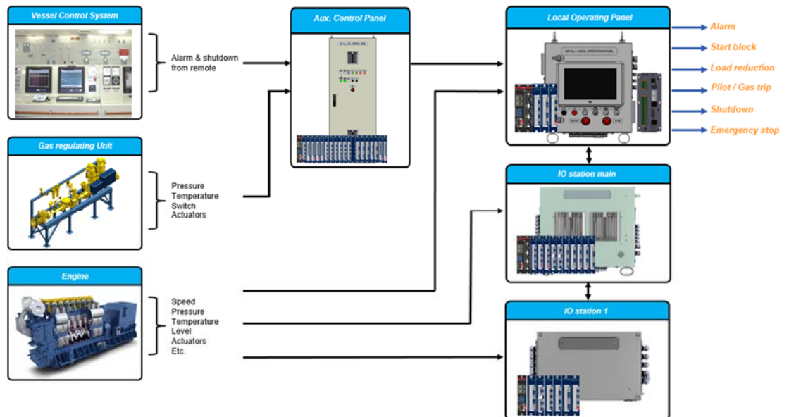
Figure 5.13 Engine control system safety function
