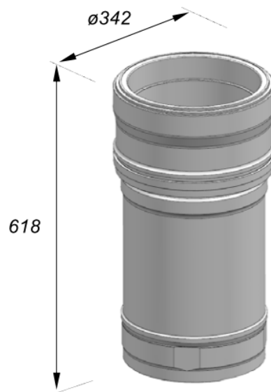
Cylinder liner (Weight : approx. 85 kg)
