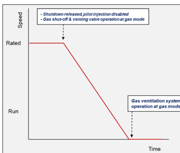
Figure 5.12 Emergency stop sequence
