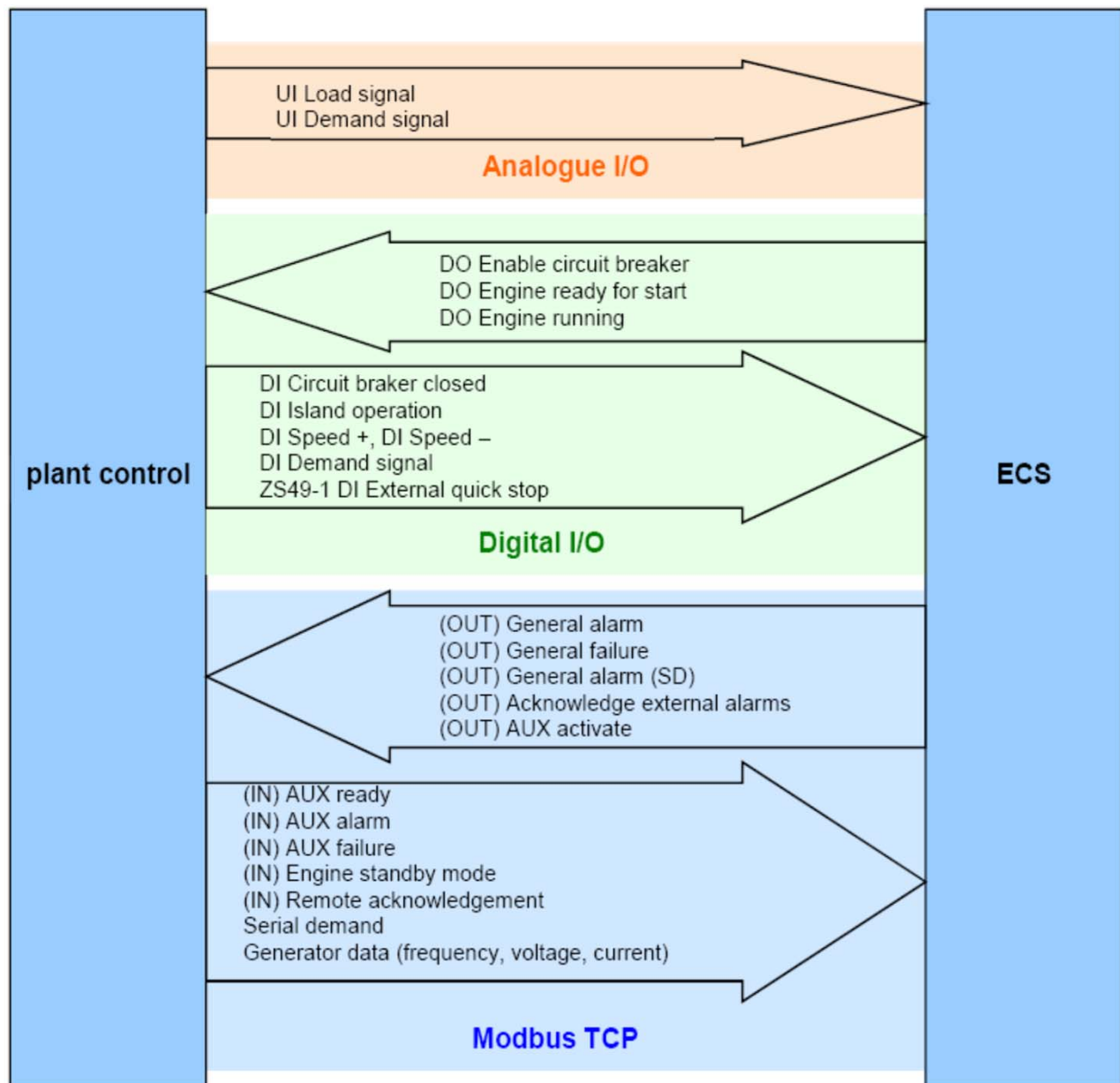
Fig. 4-3-2 Hardwire Interface
