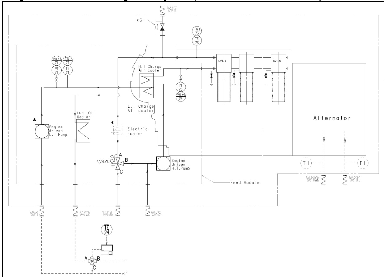
Diagram for internal cooling water system (HTCW : Air cooler to Jacket)
