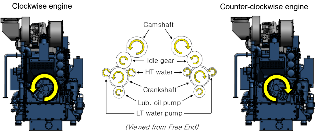
Figure 1.2 Direction of engine rotation
