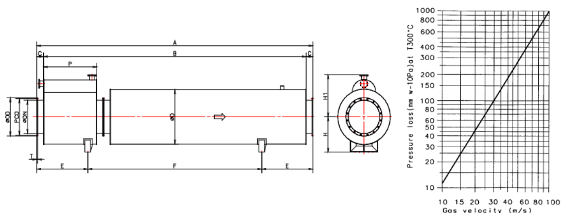
Figure 9.5 Exhaust gas silencer (25 dB type)
