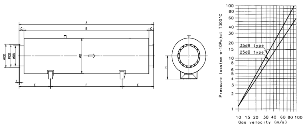
Figure 9.8 Exhaust gas silencer (35 dB type).
