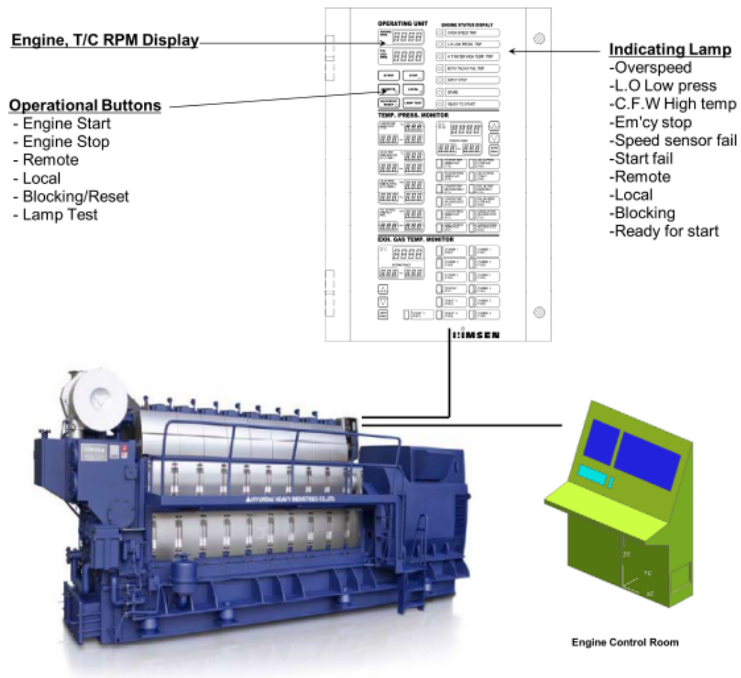
Figure 5.3 HiMSEN engine control communication interface
