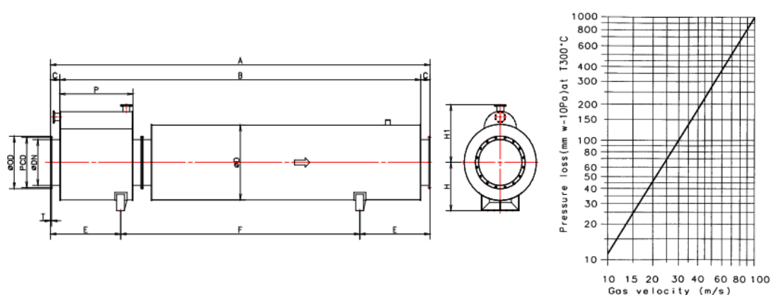
Figure 9.6 Exhaust gas silencer (35 dB type).
