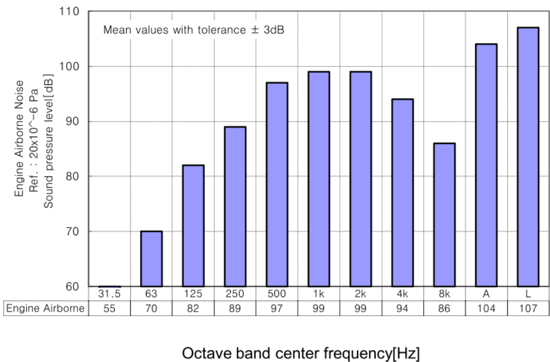
Figure 4.1 Engine air airborne noise level (720 rpm)
