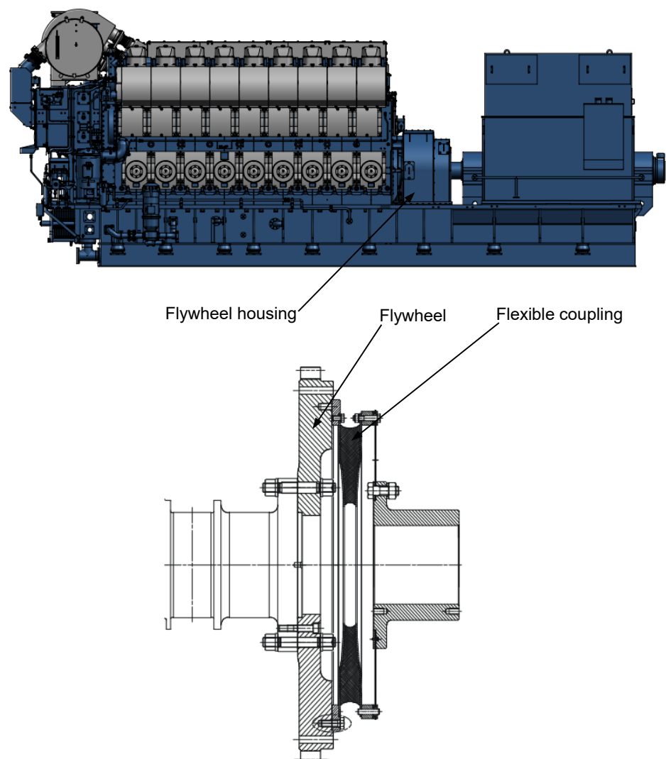
Figure 9.9 Flexible coupling outline
