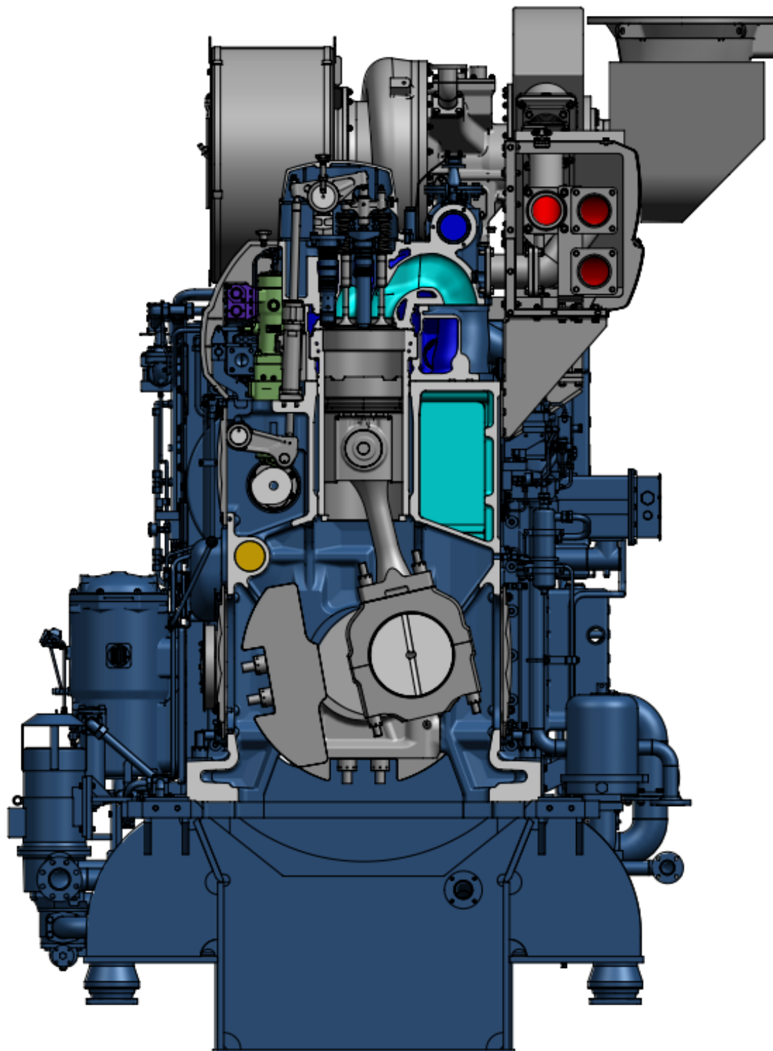
Figure 2.1 Engine cross section
