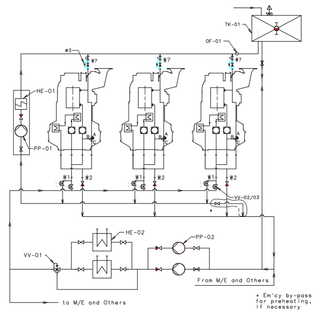
Figure 8.3 Diagram for external cooling water system-1 (pre-heating unit)
