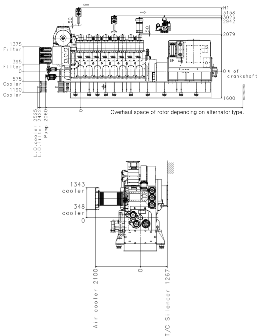
Figure 2.7 Overhaul dimension
