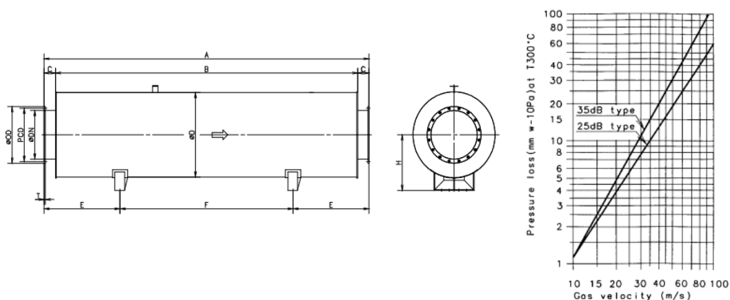
Figure 9.7 Exhaust gas silencer (25 dB type).
